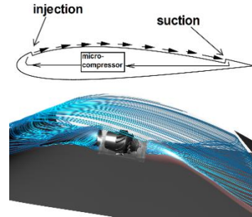
Figure 1. CFJ Injection and Suction [20,19,3]
