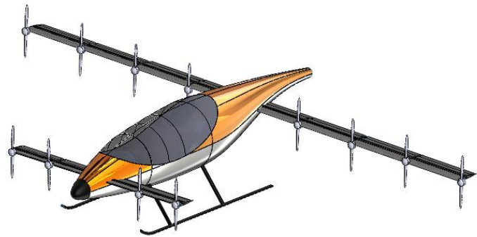
Figure 5. Martian eVTOL Colibri Aircraft Model
