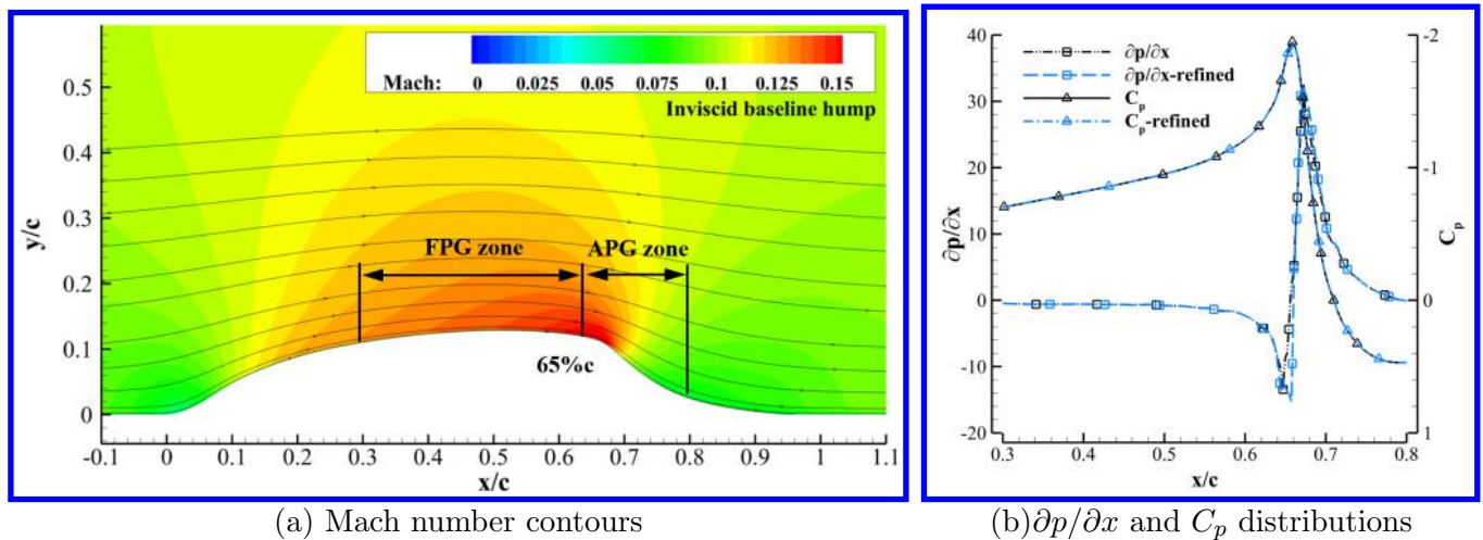
Figure 4: Results of the baseline hump with inviscid flow simulation.
