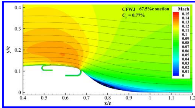
(a) Case 8, suction at 67.5% c
