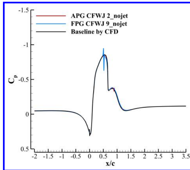
Figure 21: C_p distributions for the baseline and the optimum CFWJ cases with no jet.
