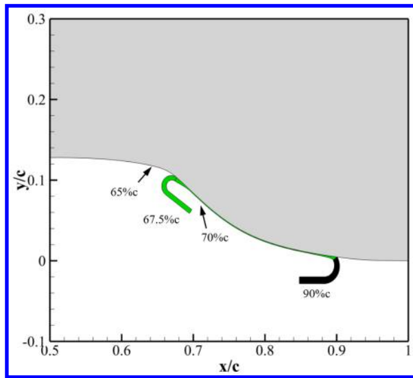
Figure 7: Injection location trade study (Case 1, 2, 3).
