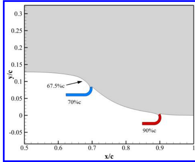
Figure 26: Suction location trade study (suction-only Case 1, 2 and 3).
