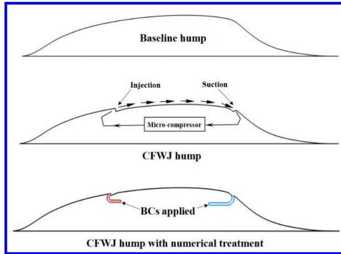
Figure 6: Sketch of the CFWJ hump.
