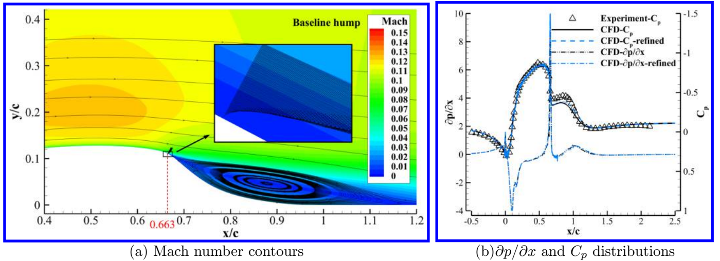
Figure 5: Results of the viscous baseline hump.
