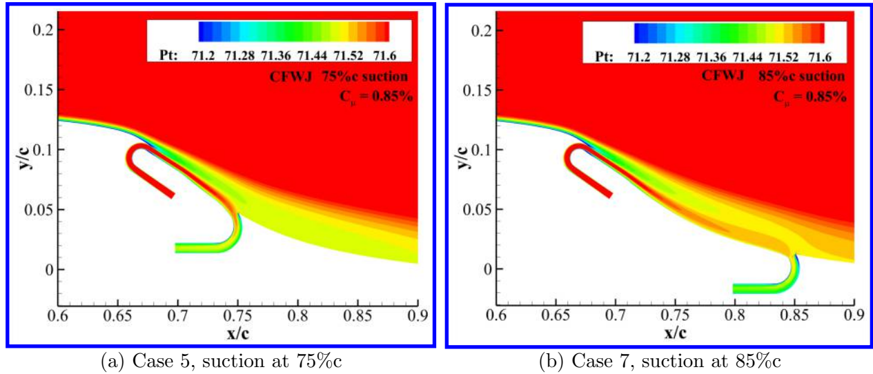
Figure 11: Total pressure comparison with the injection fixed at 67.5%c.
