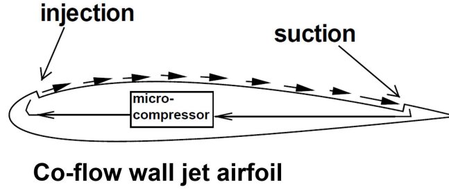
Figure 1: Schematics of the CFWJ airfoil.
