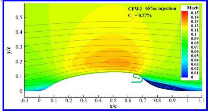
(c) Case 16, injection at 65% c
