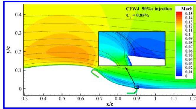
Figure 25: Streamlines of CFWJ Case 2 with zoomed view to show VP difference at Stations 4 and 5.
