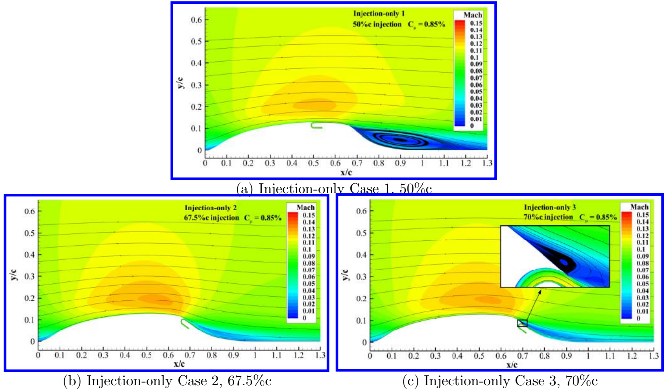
Figure 23: Injection-only trade study.
