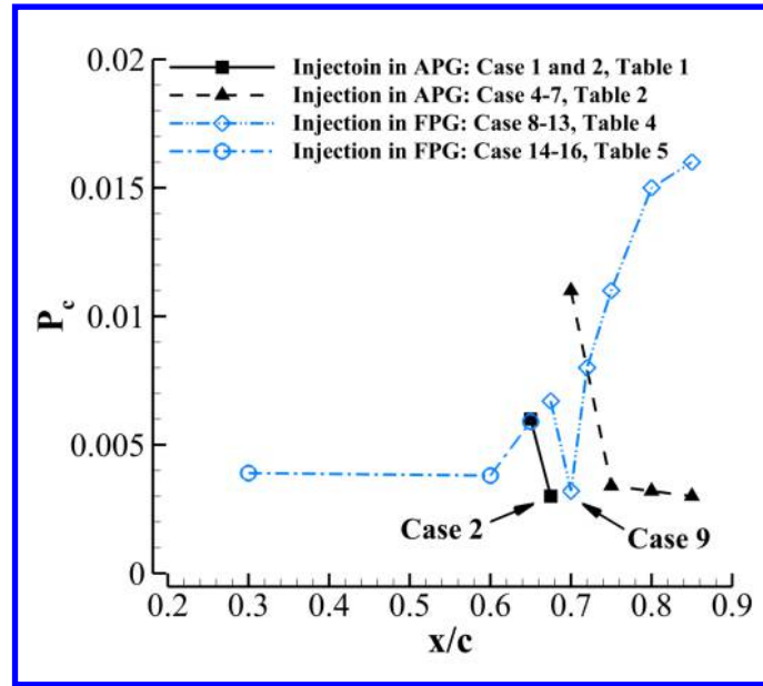
Figure 17: Power coefficient versus locations.
