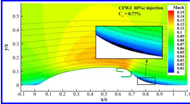
(b) Case 15, injection at 60% c
