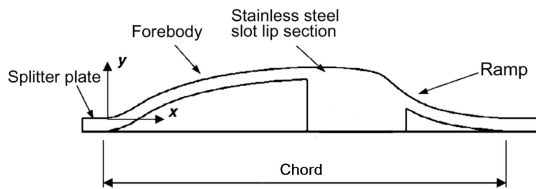
Figure 3: Geometry of the hump upper surface [50].
