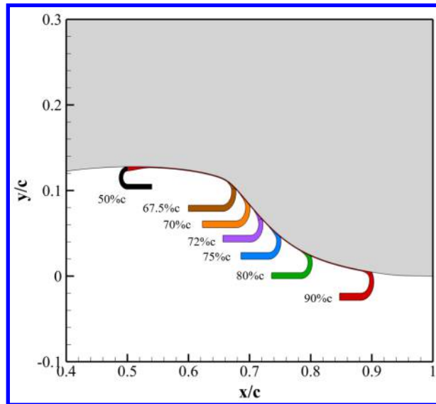
Figure 12: Suction location trade study (Case 8-13).
