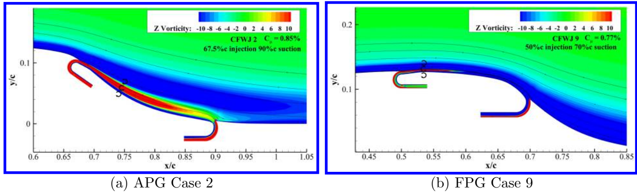
Figure 20: Spanwise vorticity for the optimum FPG and APG cases.
