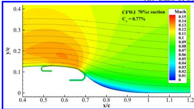
(b) Case 9, suction at 70% c
