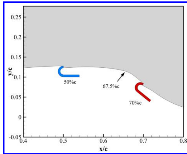
Figure 22: Injection location trade study (injection-only Case 1, 2 and 3).
