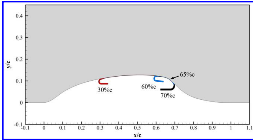
Figure 15: Injection location trade study (Case 14, 15, and 16).
