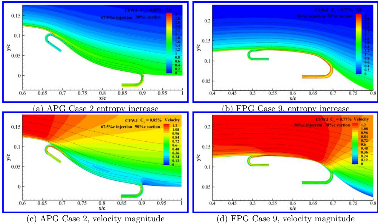
Figure 19: Comparison between the optimum APG and FPG cases.
