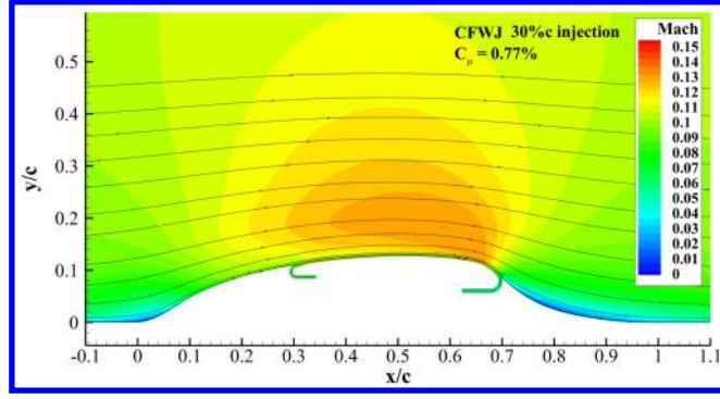
(a) Case 14, injection at 30% c
