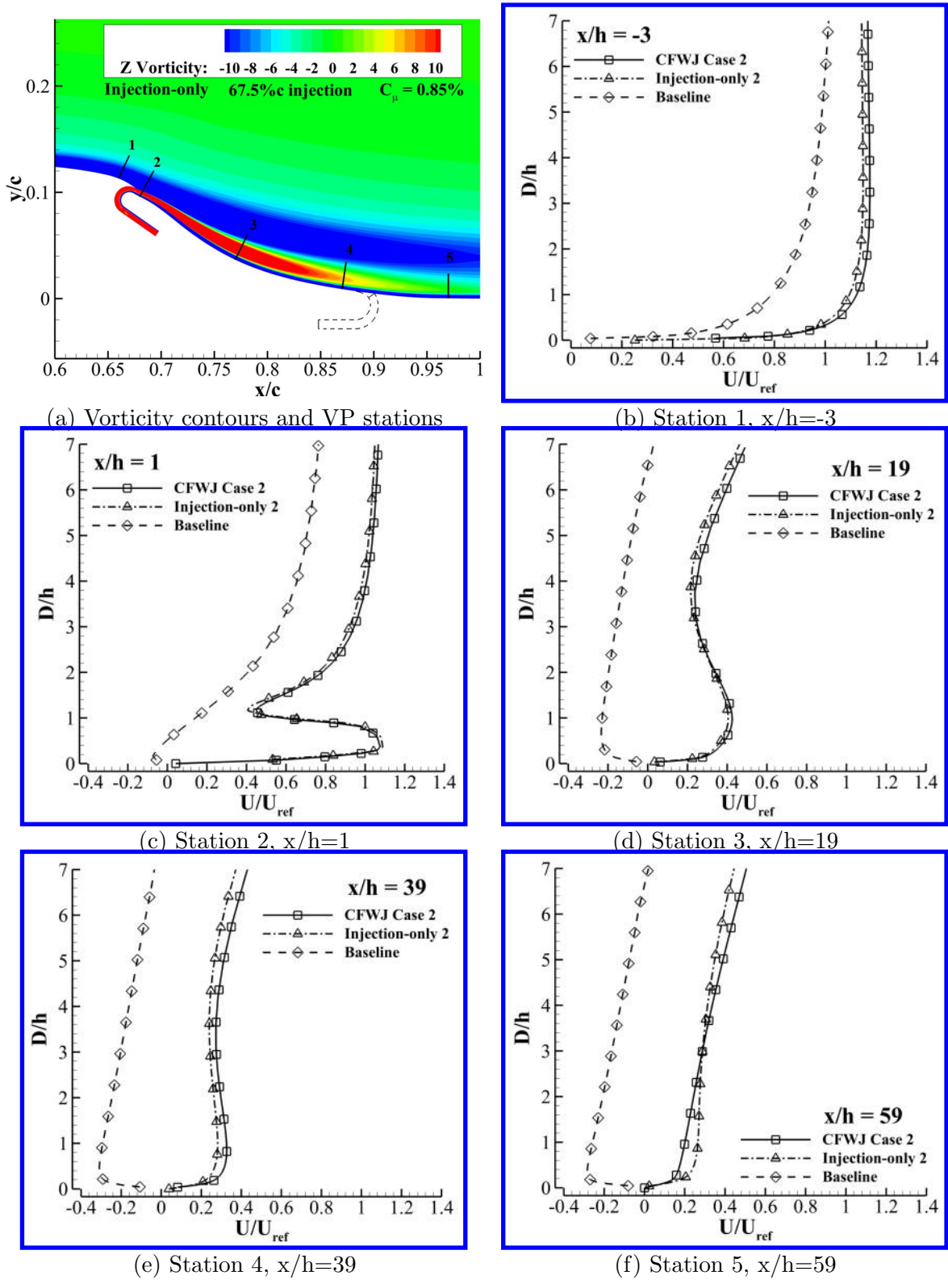
Figure 24: The spanwise vorticity of the injection-only Case 2 and the velocity profiles compared with the CFWJ Case 2.
