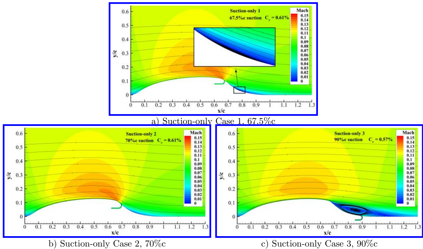
Figure 27: Suction-only trade study.
