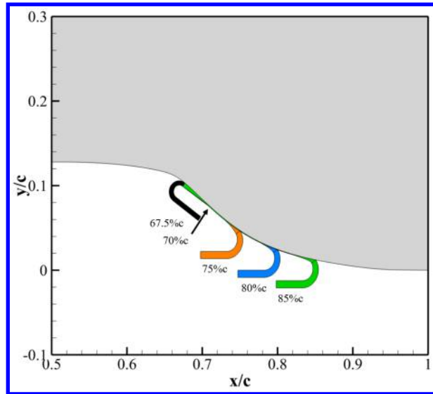
Figure 9: Suction location trade study (Case 4, 5, 6, 7).
