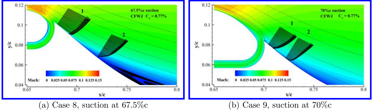
Figure 14: Mach number contours and velocity profiles.
