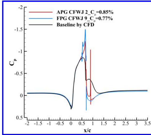
Figure 18: C_p distributions for the baseline and the optimum CFWJ cases.
