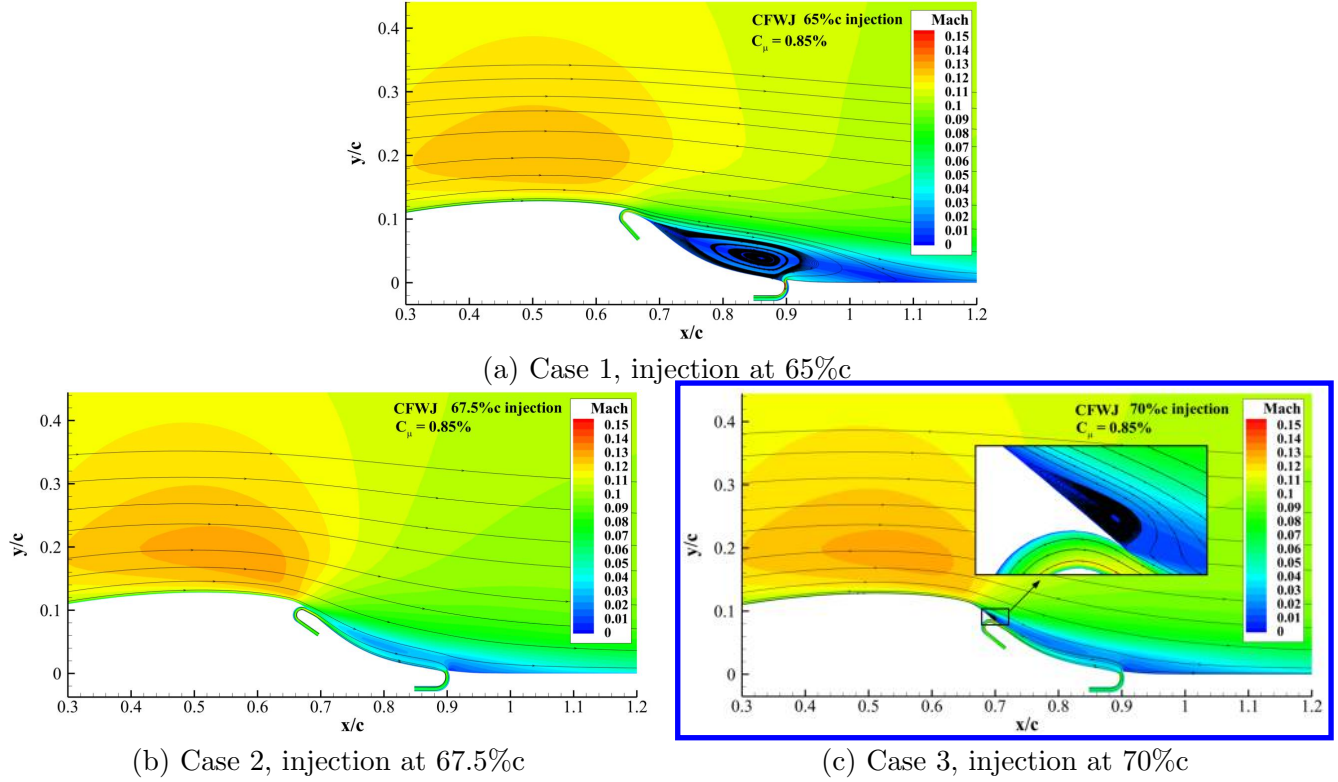
Figure 8: Injection location trade study with the suction fixed at 90%c position.
