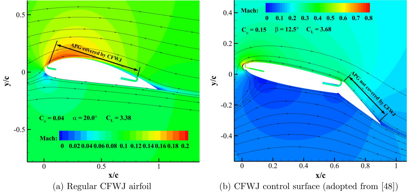
Figure 2: Mach number contours of CFWJ applications.
