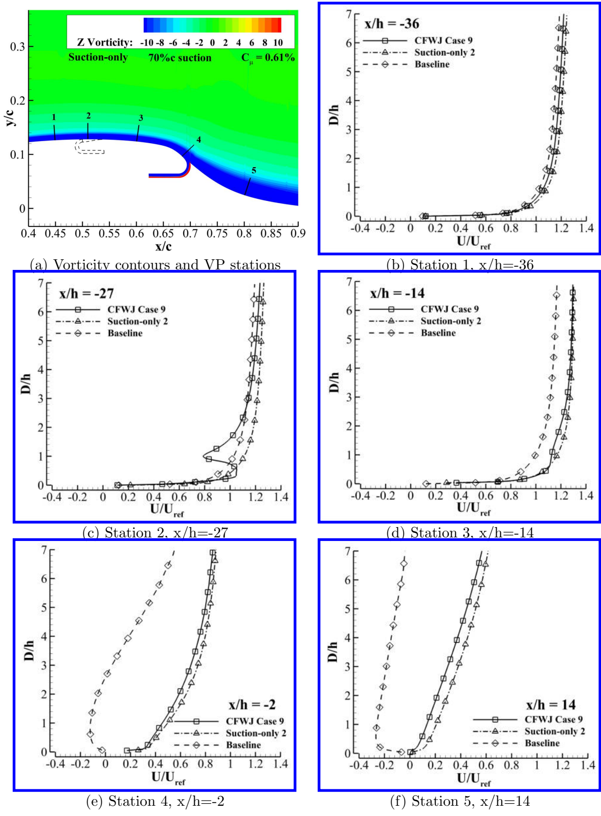
Figure 28: The spanwise vorticity of the suction-only Case 2 and the velocity profiles compared with the CFWJ Case 9.
