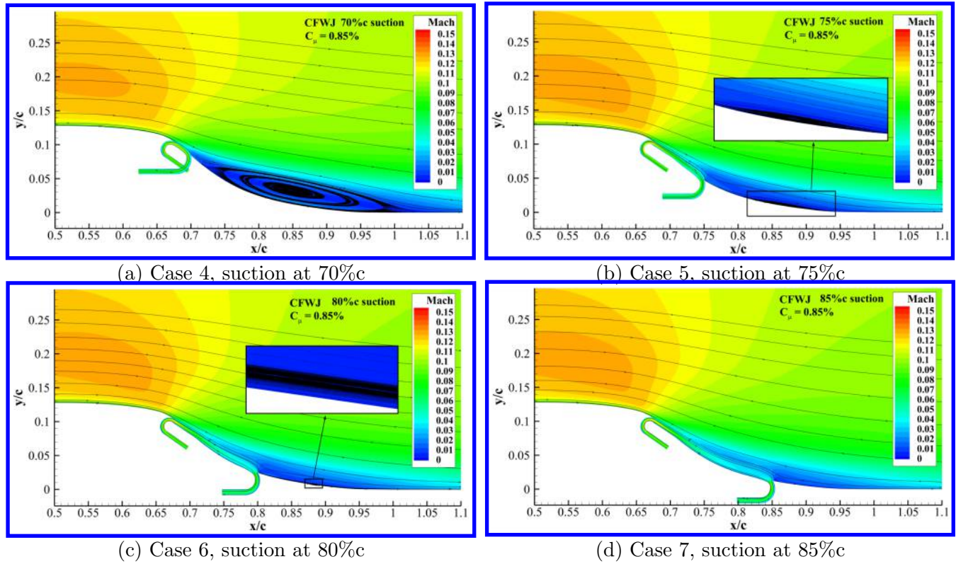
Figure 10: Suction location trade study with the injection fixed at 67.5% c position.
